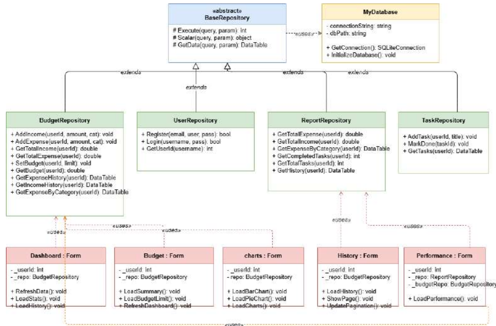
Figure 2.4: Class Diagram
